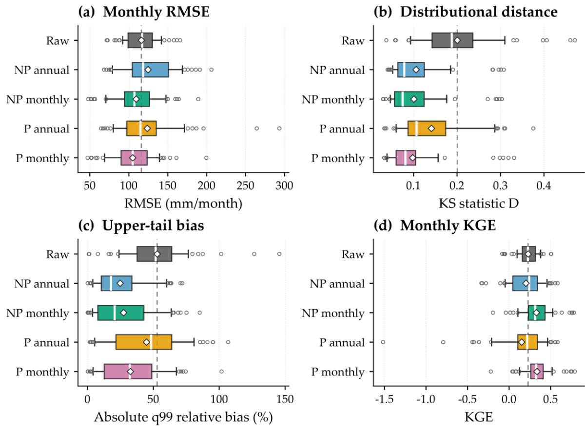
Figure 4. Validation distributions for 60 model-station combinations per variant. Boxes show the interquartile range, whiskers show the 10th-90th percentiles, diamonds show means, centre lines show medians, and dashed vertical lines show the raw mean in each panel; these are not bootstrap distributions.
